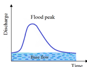
Figure 1 – Floods propagation
