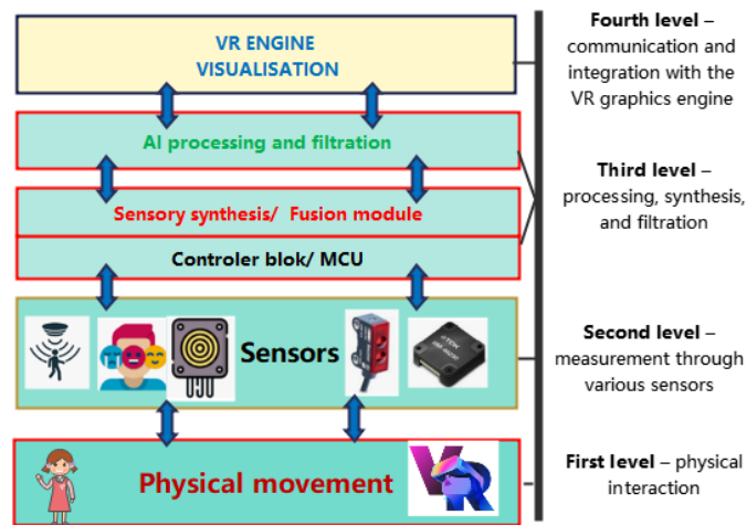
Figure 1-VR sensor system architecture
