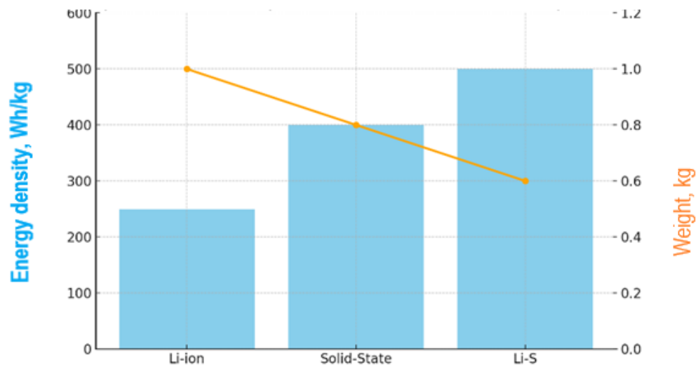
Figure 2 – Energy density of the main types of batteries for mobile robots
