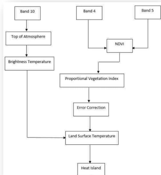
Figure 2 – Methodology to calculate the urban heat islands (Opong J., 2021)
