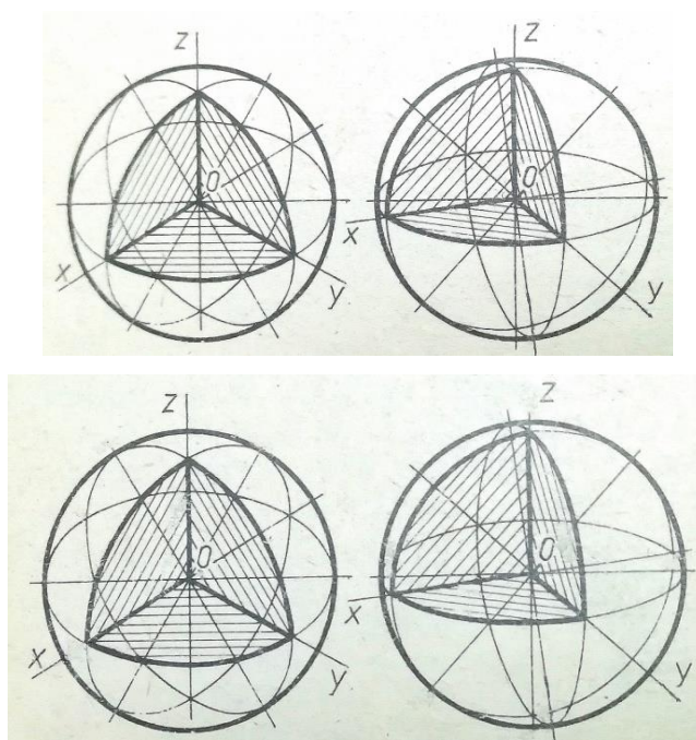
Fig. 1. An example for the development of creative thinking
