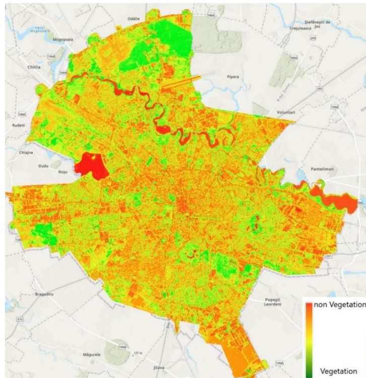
Figure 3 – Classified raster of the Normal difference vegetation index
