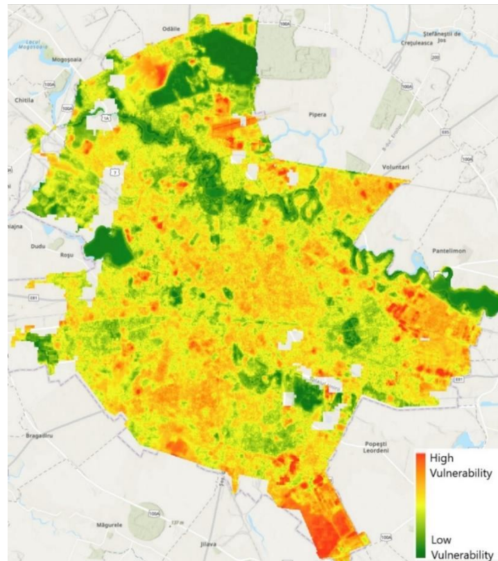
Figure 5 – Vulnerability to high temperatures inside the city of Bucharest
