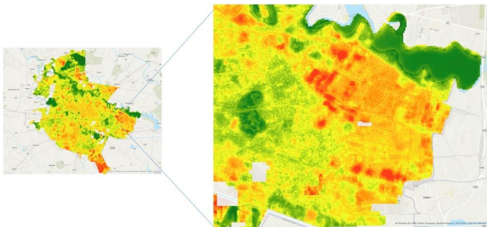
Figure 6 – Urban heat islands in the city of Bucharest
