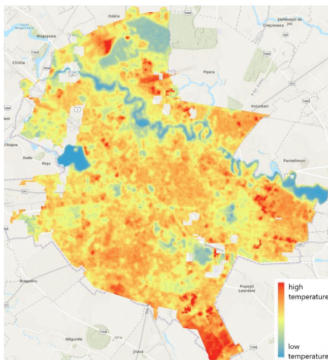
Figure 4 – Classified raster with the values of the Brightness temperatures over the city of Bucharest
