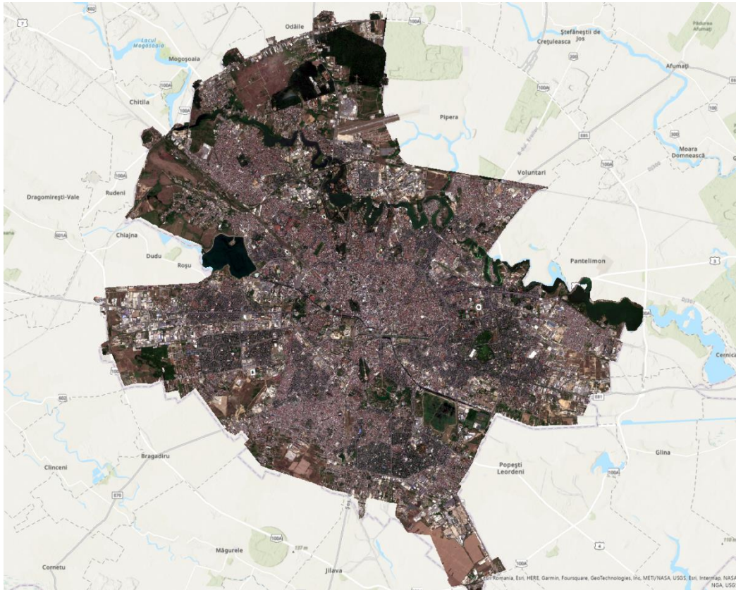
Figure 1 – Satellite image cropped to the administrative boundaries of the city of Bucharest
